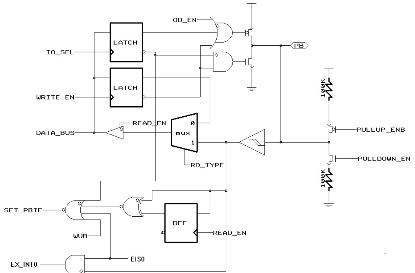
Figure 10 Block Diagram of PB0
