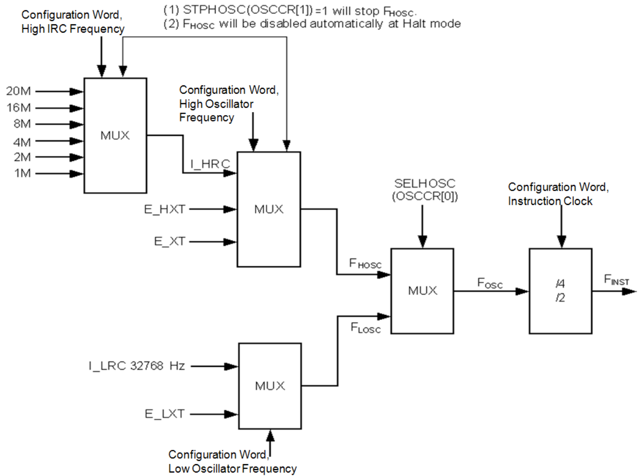
Figure 34 Oscillation Configuration of NY8B062D
