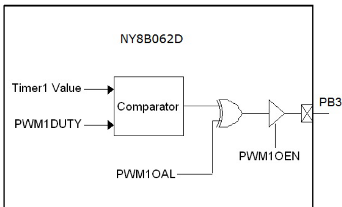
Figure 18 PWM1 Block Diagram
